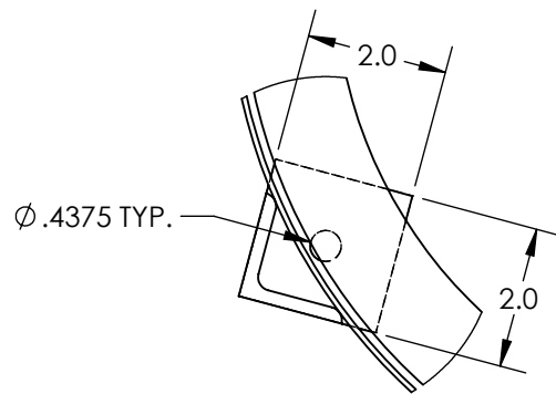
DETAIL A SCALE 1 : 3
