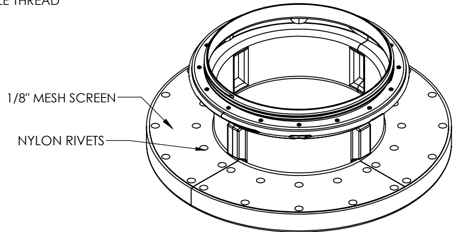
BOTTOM SIDE VIEW
