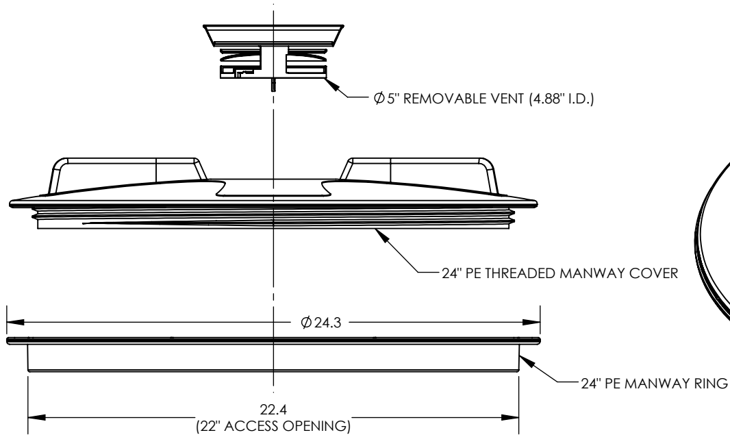
EXPLODED VIEW
