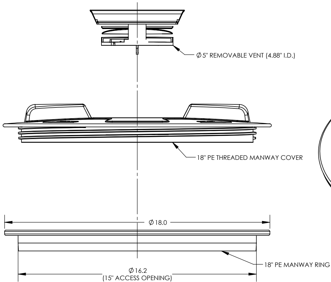
EXPLODED VIEW
